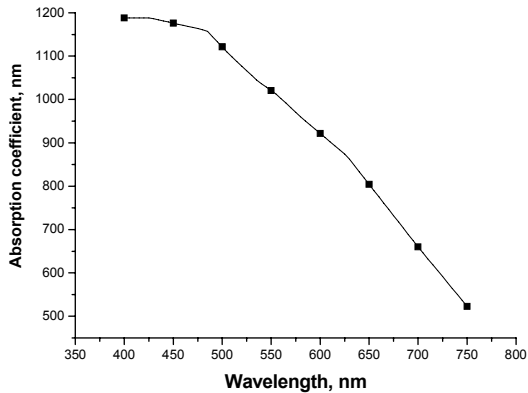
Figure 4: The absorption properties of retinal pigment epithelium 25
