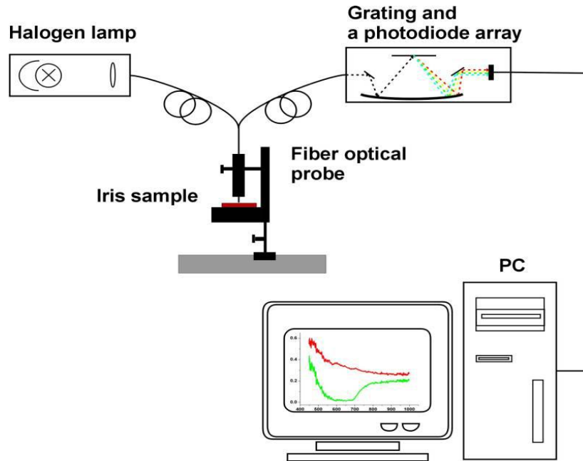
Figure 6: Experimental setup for in vitro measurements
