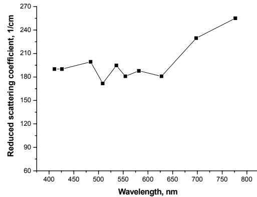
Figure 5: The scattering properties of retinal pigment epithelium 25
