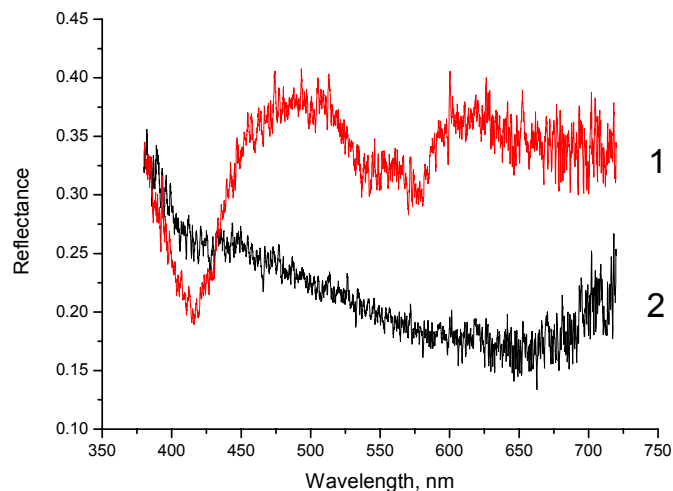
Figure 10: The typical reflectance spectra of rabbit irises. 1 - the reflectance spectrum of vitiligo iris; 2 - the reflectance spectrum of brown iris of a rabbit.
