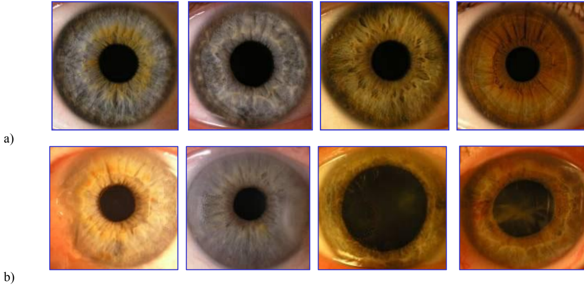
Figure 8: Digital in vivo images of (a) healthy and (b) primary open angle glaucoma human eyes
