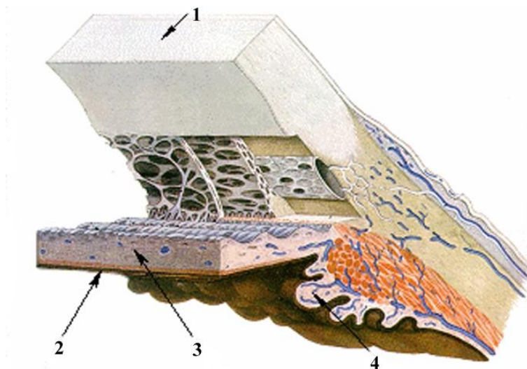
Figure 2: The eye iris structure: 1 - the cornea; 2 - the iris pigment epithelium (IPE); 3 - the iris stroma; 4 - the ciliary body
