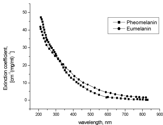
Figure 3: Extinction coefficient spectra of melanins 24
